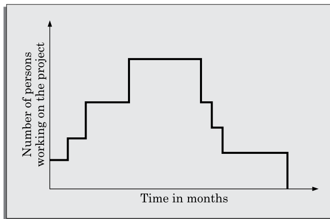
FIGURE 3.3 Person-month curve.
