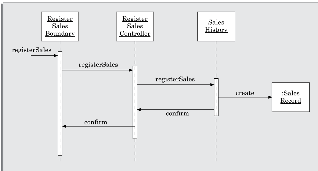
FIGURE 8.20 Sequence diagram for the register sales use case of Example 8.3.
