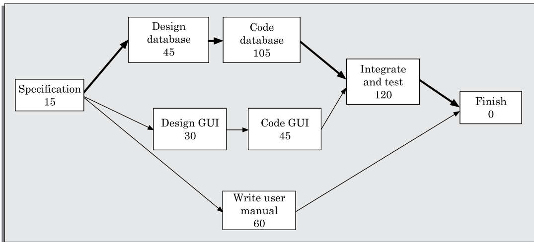
FIGURE 3.9 Activity network representation of the MIS problem.
