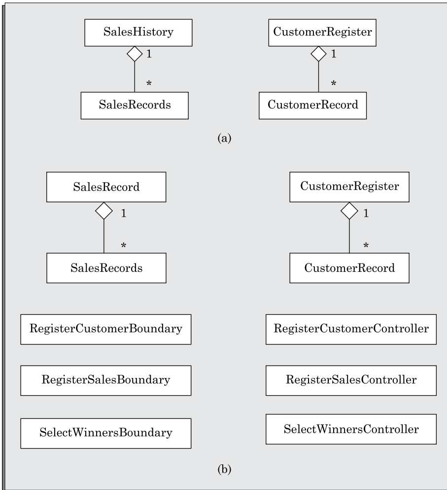
FIGURE 8.17 (a) Initial domain model (b) Refined domain model for Example 8.3.
