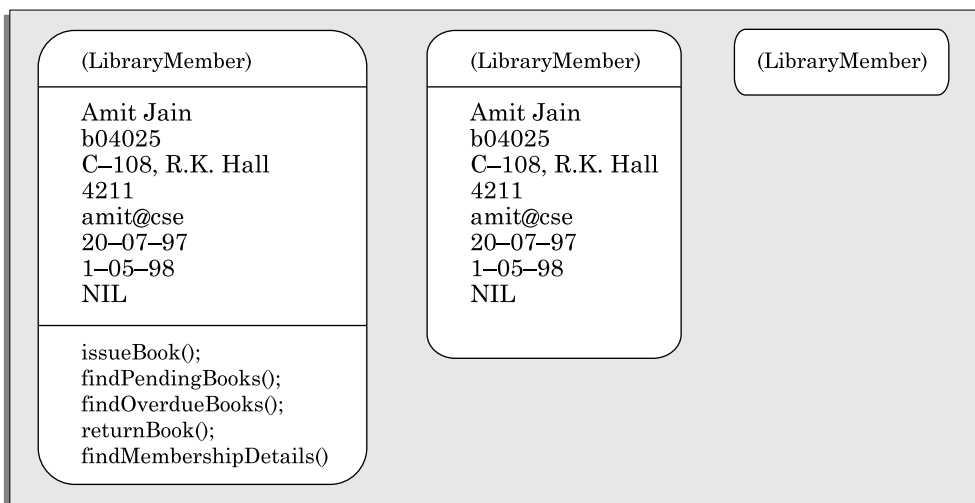
FIGURE 7.29 Different representations of a LibraryMember object.
