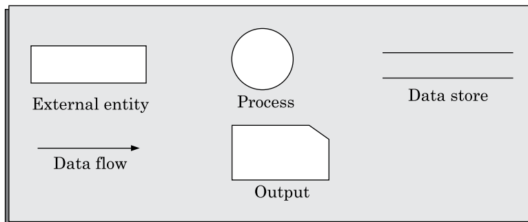
FIGURE 6.2 Symbols used for designing DFDs.
