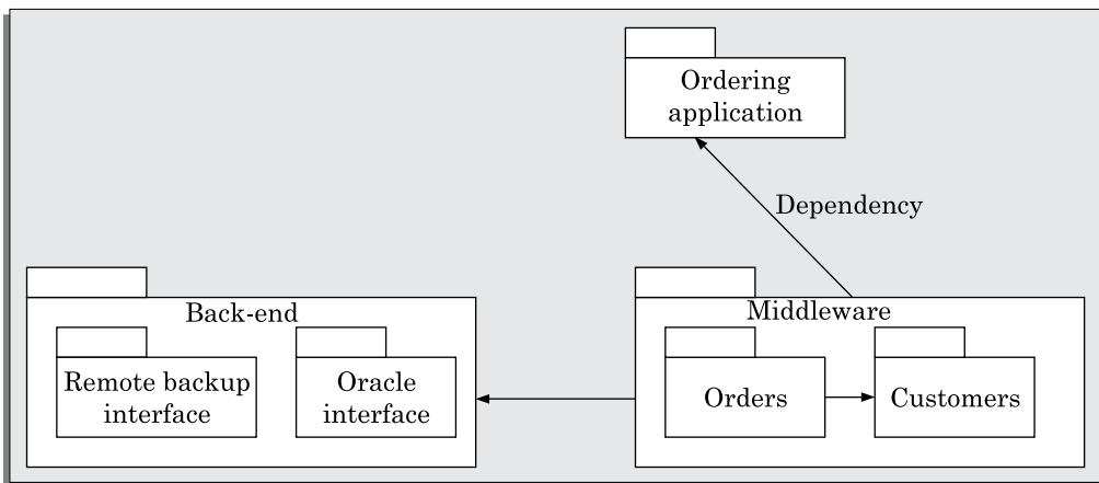
FIGURE 7.34 An example package diagram.
