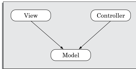
FIGURE 8.4 Class structure for the MVC pattern.
