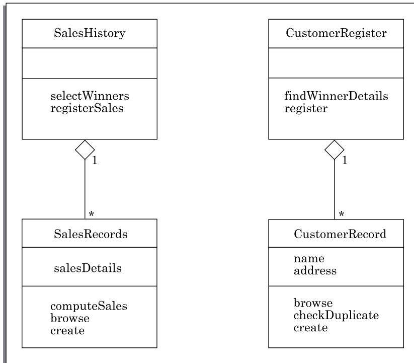
FIGURE 8.22 Class diagram for Example 8.3.
