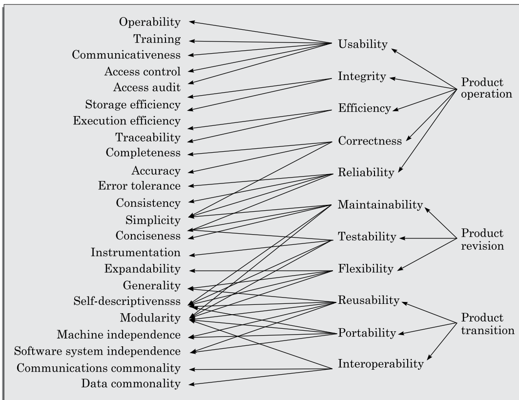
FIGURE 11.4 McCall's quality model.
