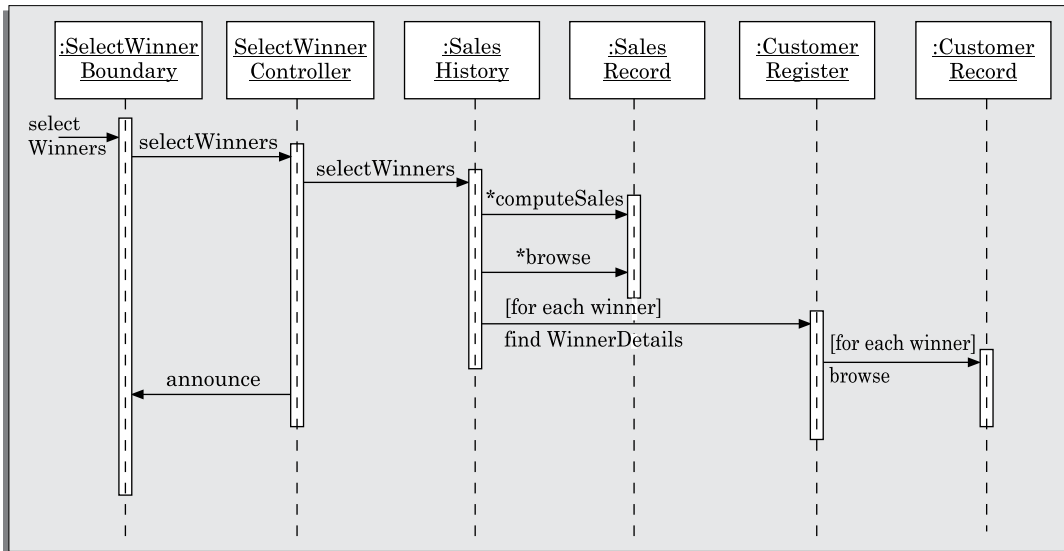
FIGURE 8.18 Sequence diagram for the select winner list use case of Example 8.3.
