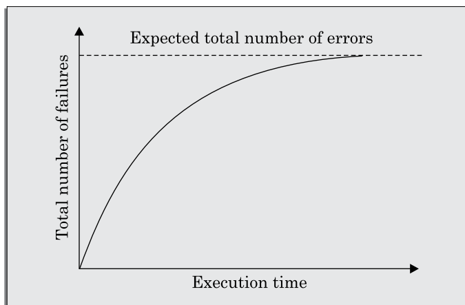
FIGURE 11.3 Goel-Okutomo reliability growth model.
