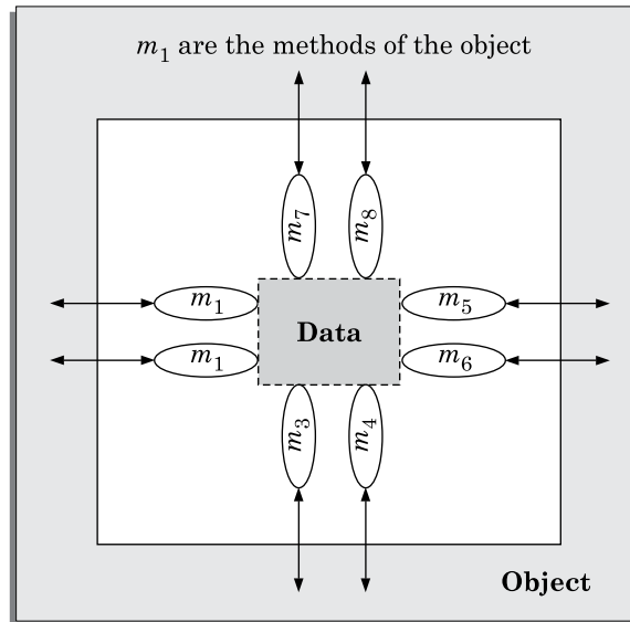
FIGURE 7.2 A model of an object
