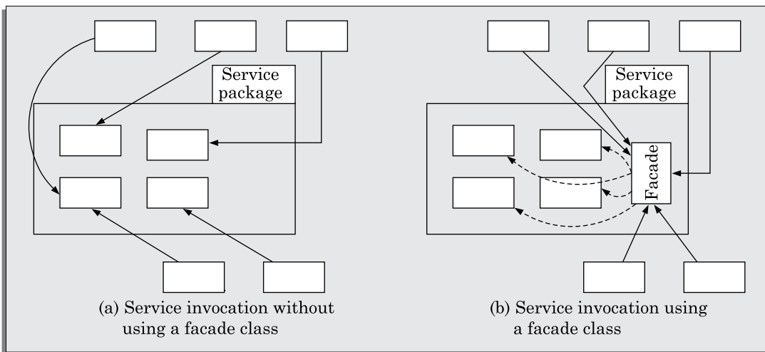
FIGURE 8.2 Service invocation with and without using a facade class.
