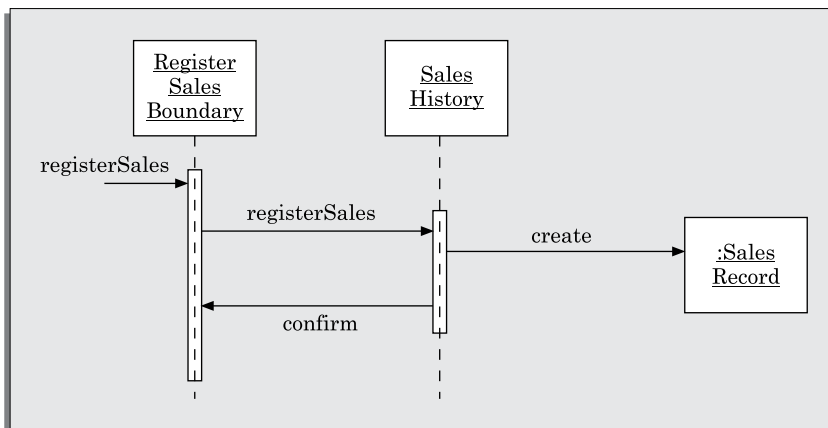
FIGURE 8.21 Refined sequence diagram for the register sales use case of Example 8.3.
