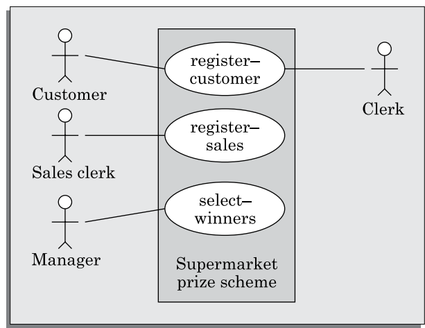
FIGURE 8.16 Use case model for Example 8.3.
