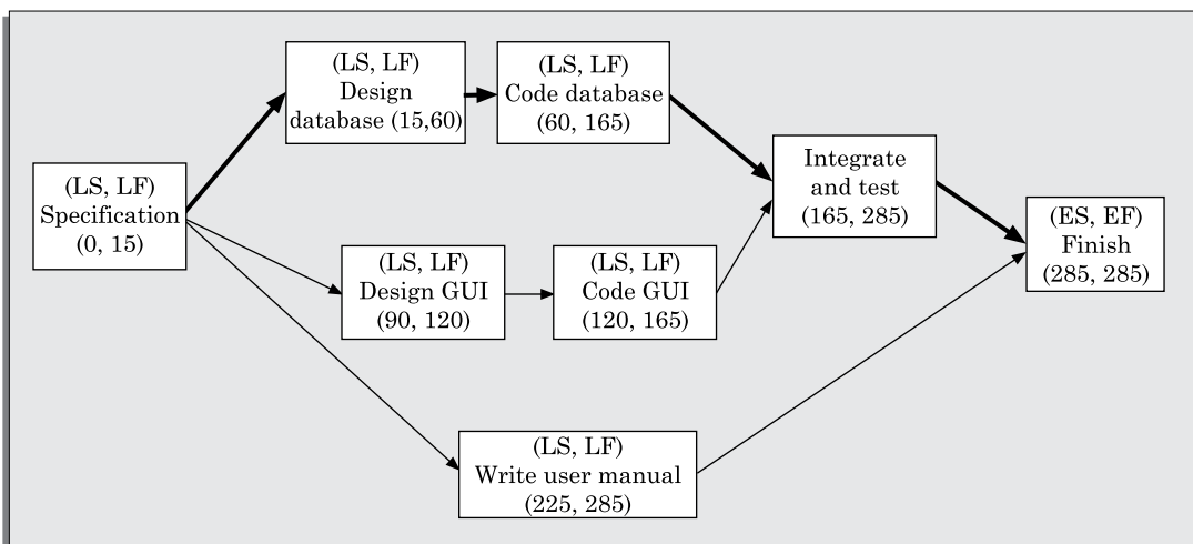
FIGURE 3.11 AoN of MIS problem with (LS, LF).
