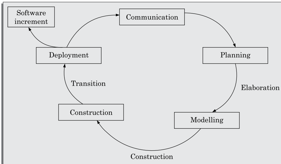
FIGURE 8.8 Unified process model.
