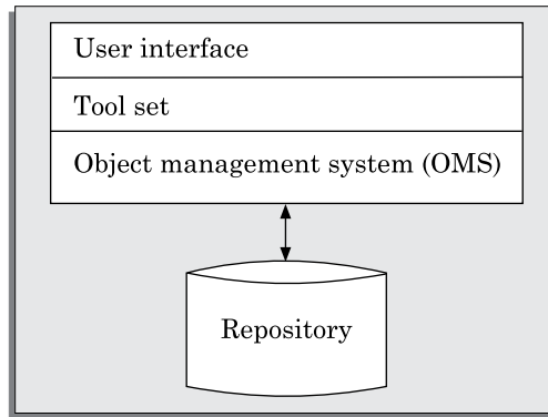
FIGURE 12.2 Architecture of a modern CASE environment.
