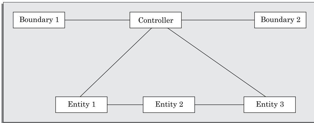
FIGURE 8.10 A typical realisation of a use case through the collaboration of boundary, controller, and entity objects.
