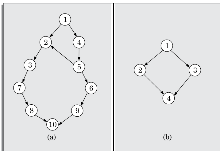
FIGURE 1.10 Control flow graphs of the programs of Figures 1.9(a) and (b).
