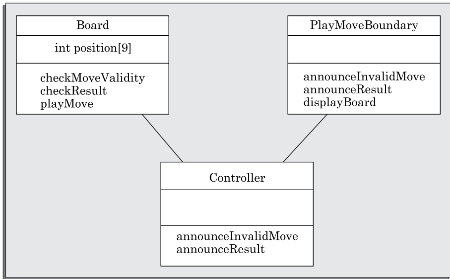
FIGURE 8.15 Class diagram for Example 8.2.
