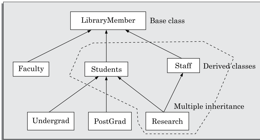
FIGURE 7.4 An example of multiple inheritance.
