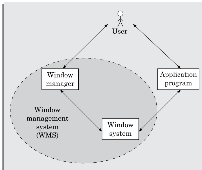
FIGURE 9.4 Window management system.
