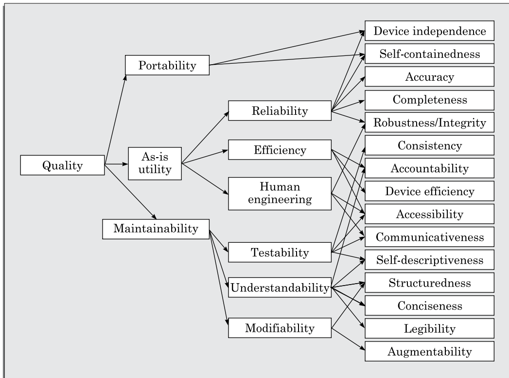
FIGURE 11.6 Boehm's quality model.
