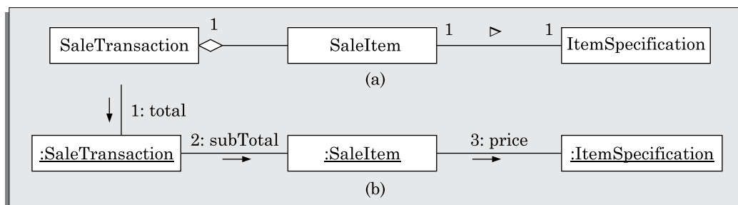
FIGURE 8.1 Expert pattern: (a) Class diagram (b) Collaboration diagram.
