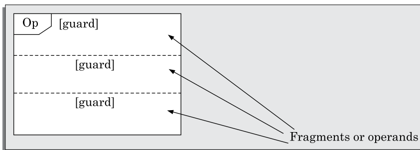
FIGURE 7.35 Anatomy of a combined fragment in UML 2.0.
