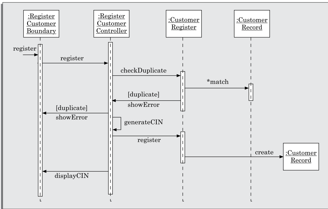
FIGURE 8.19 Sequence diagram for the register customer use case of Example 8.3.
