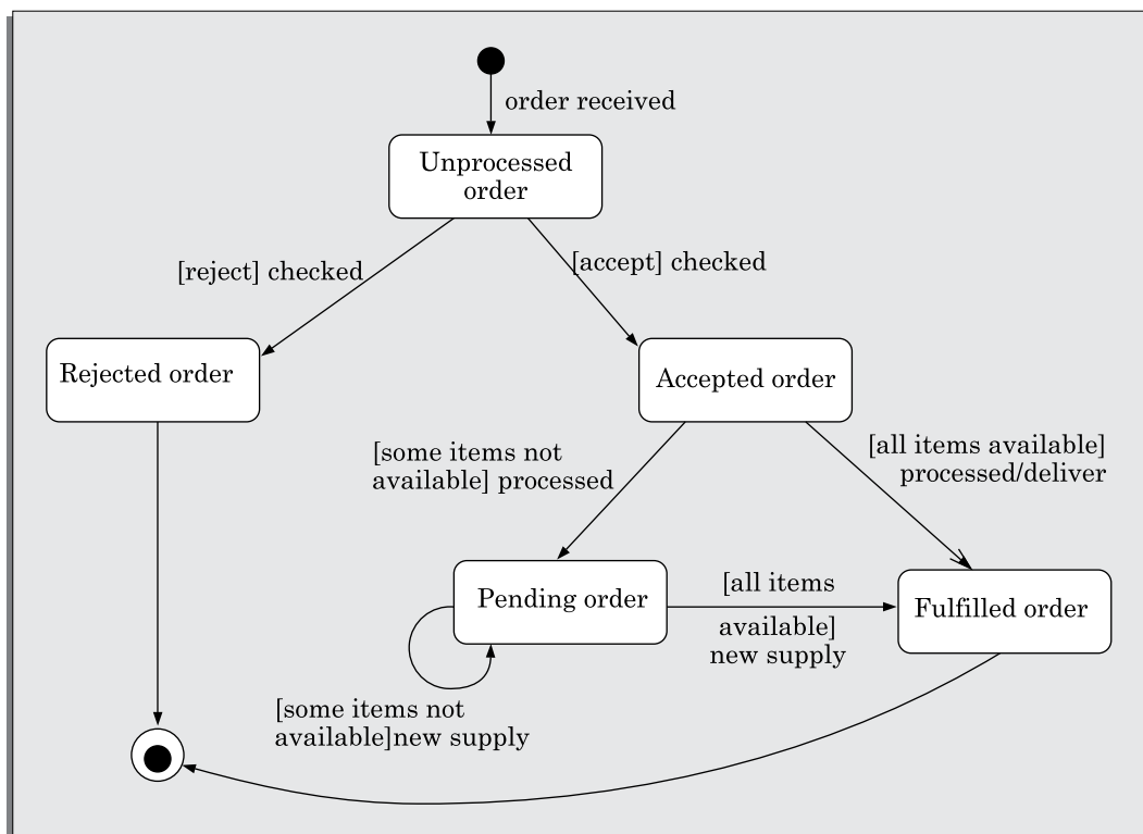
FIGURE 9.8 State chart diagram for an order object.
