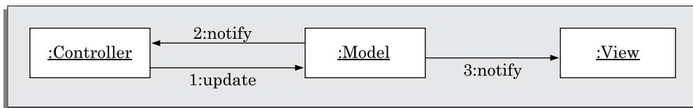
FIGURE 8.5 Interaction model for the MVC pattern.
