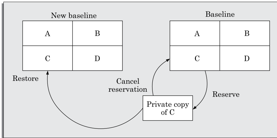
FIGURE 3.19 Reserve and restore operation in configuration control.
