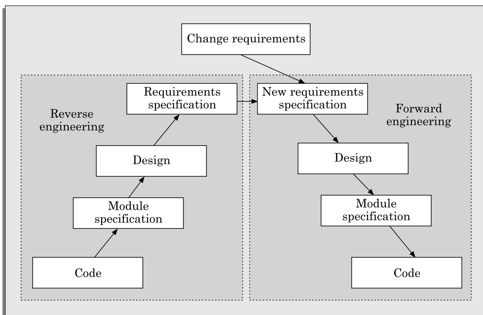
FIGURE 13.4 Maintenance process model 2.
