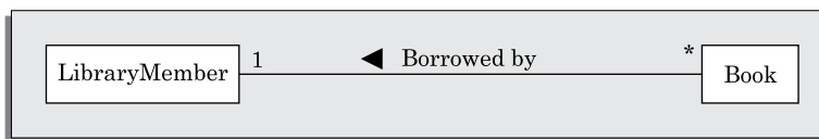
FIGURE 7.24 Association between two classes.
