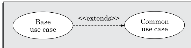
FIGURE 7.20 Example of use case extension.
