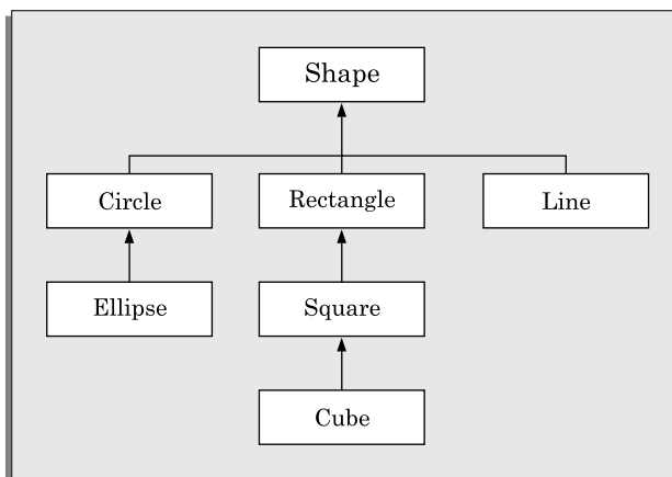
FIGURE 7.10 Class hierarchy of geometric objects.
