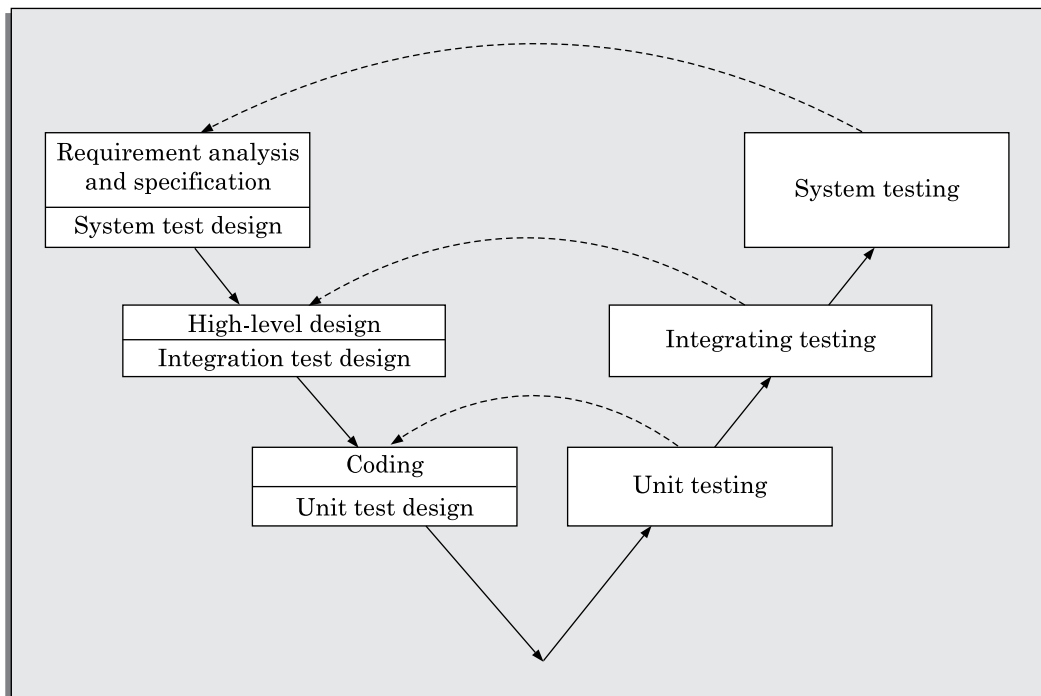
FIGURE 2.5 V-model.
