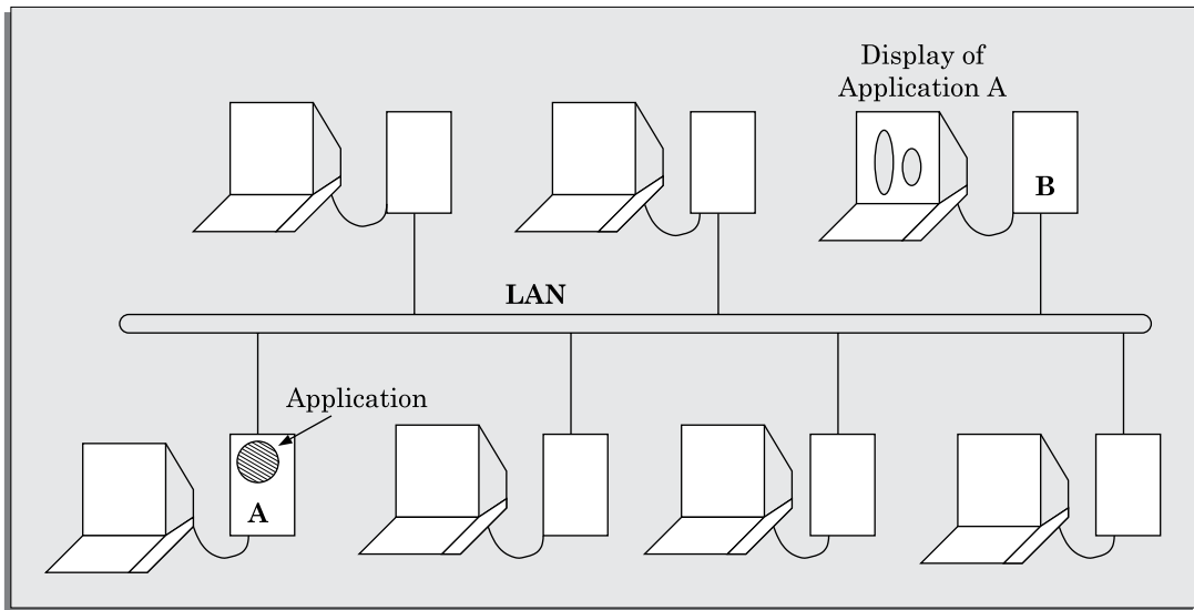
FIGURE 9.5 Network-independent GUI.
