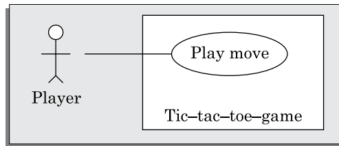
FIGURE 8.12 Use case model for Example 8.2.
