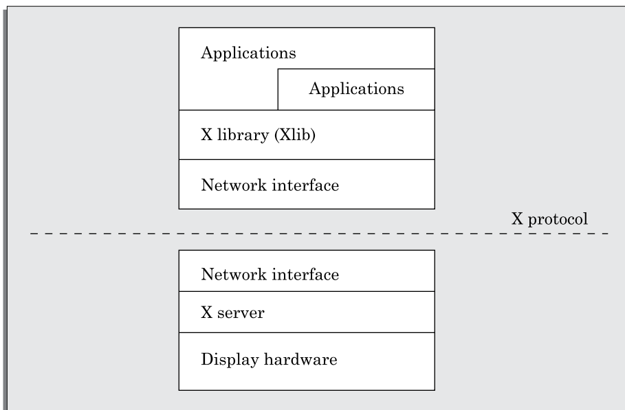
FIGURE 9.6 Architecture of the X System.
