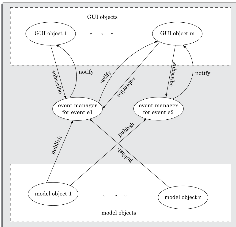
FIGURE 8.6 A schematic representation of the publish-subscribe.
