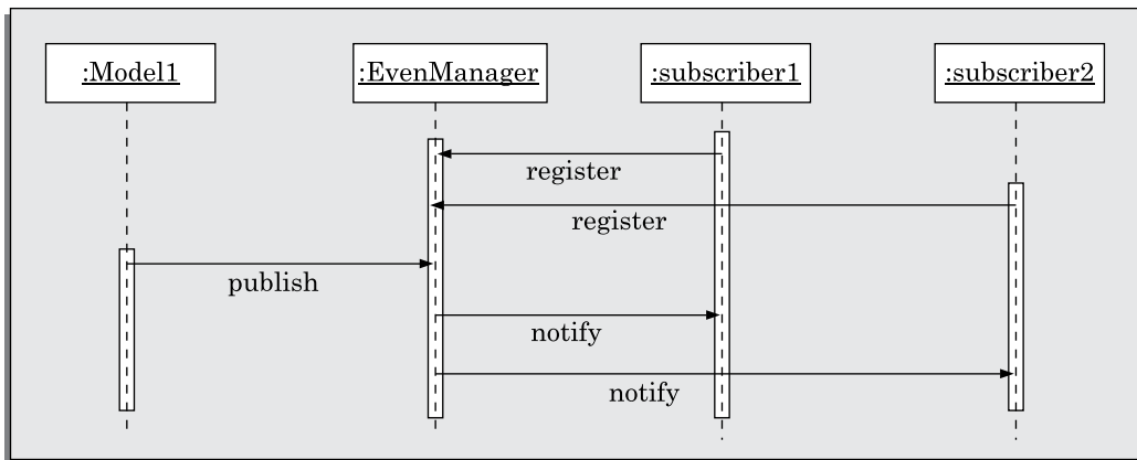
FIGURE 8.7 Interaction model of the publish-subscribe pattern.
