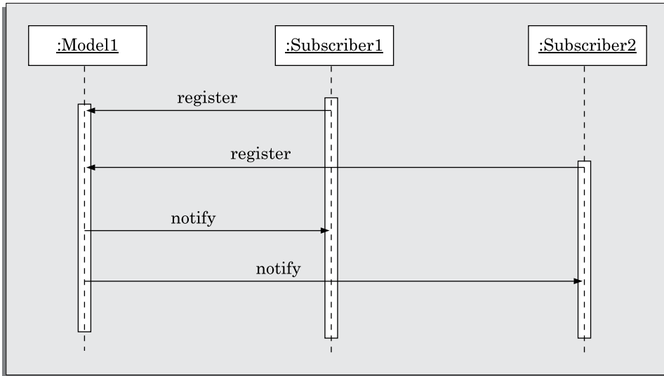
FIGURE 8.3 Interaction diagram for the observer pattern.
