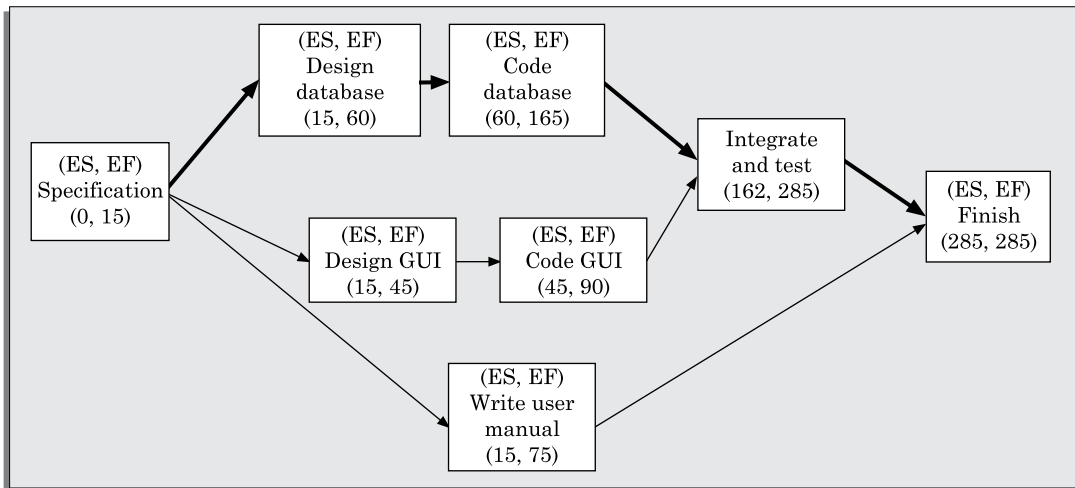
FIGURE 3.10 AoN for MIS problem with (ES, EF).
