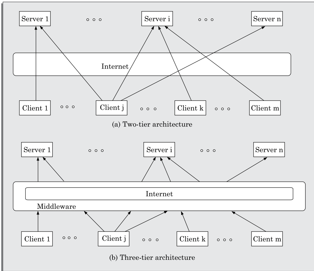
FIGURE 15.1 Two-tier and three-tier client-server architectures.
