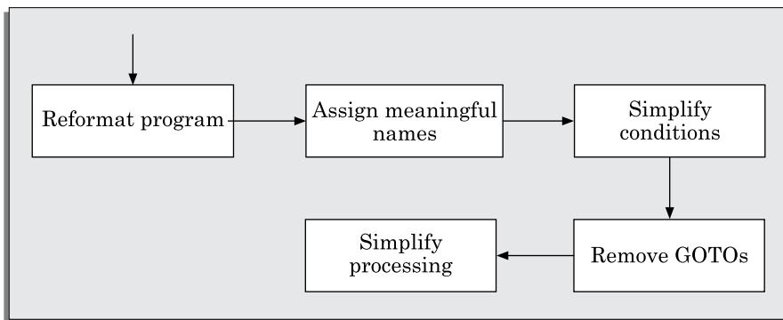
FIGURE 13.2 Cosmetic changes carried out before reverse engineering.
