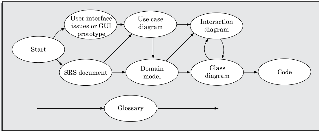
FIGURE 8.9 An object-oriented analysis and design process.
