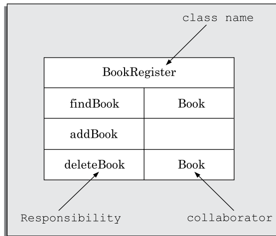
FIGURE 8.11 CRC card for the BookRegister class.
