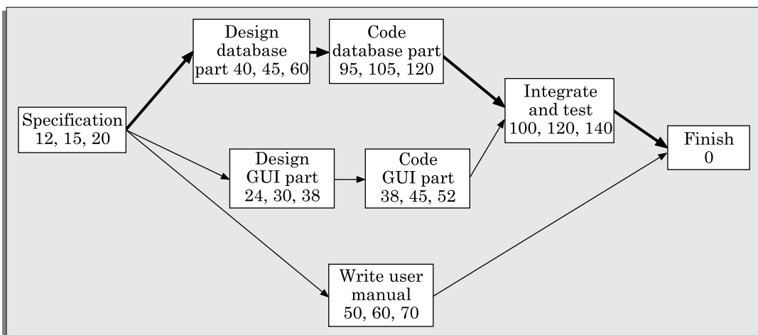
FIGURE 3.12 PERT chart representation of the MIS problem.
