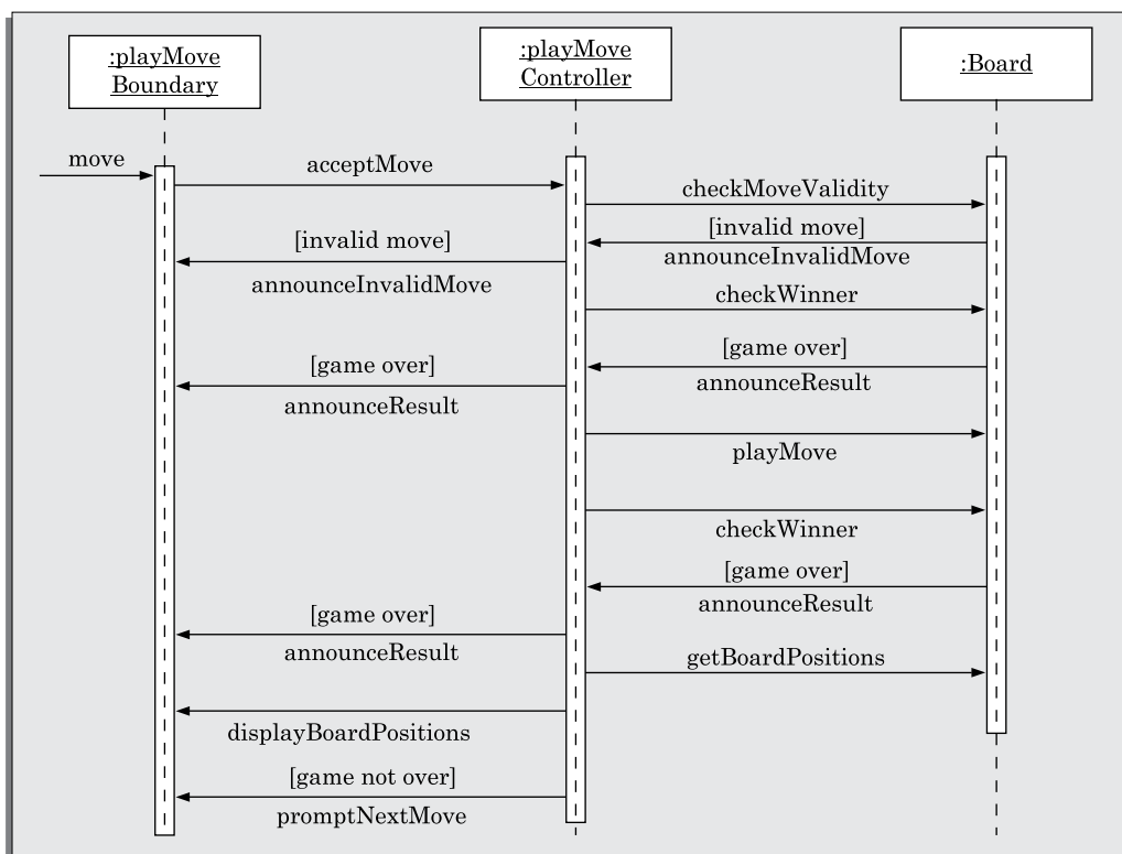
FIGURE 8.14 Sequence diagram for the play move use case of Example 8.2.
