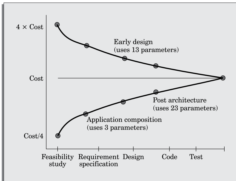
FIGURE 3.6 Accuracy of different COCOMO II estimations.
