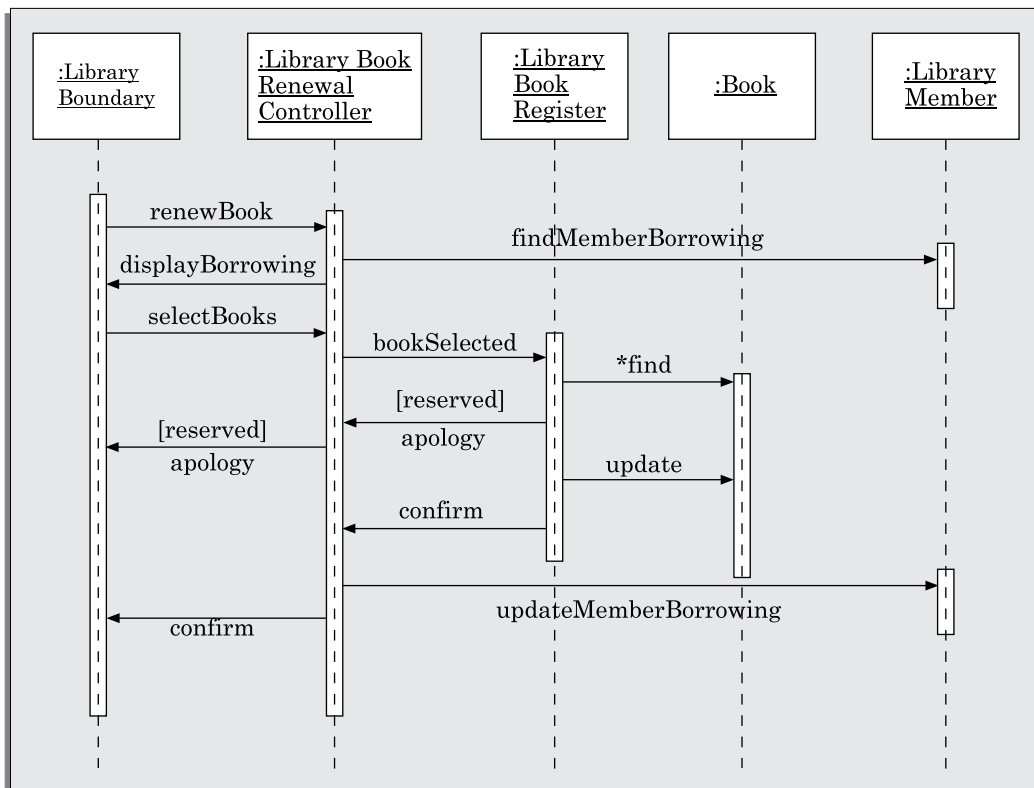
FIGURE 7.30 Sequence diagram for the renew book use case.
