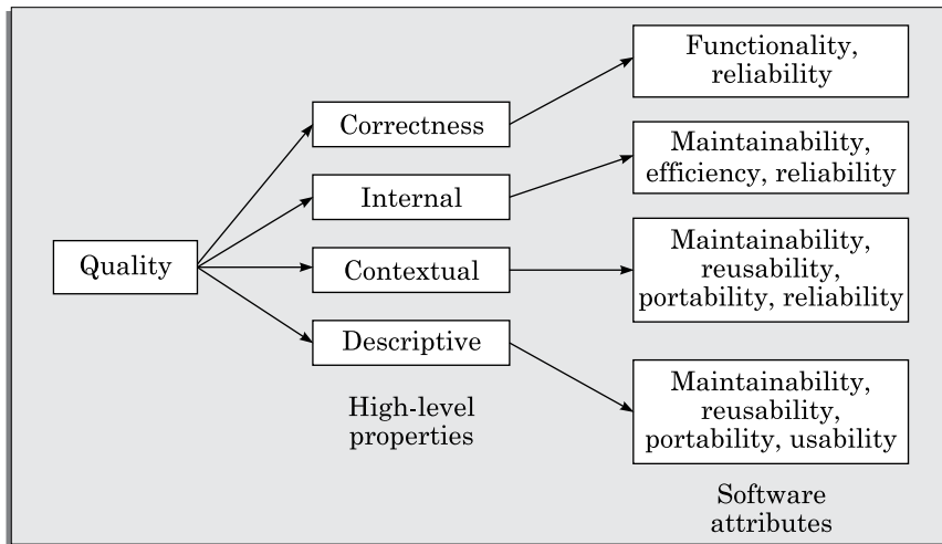
FIGURE 11.5 Dromey's quality model.
