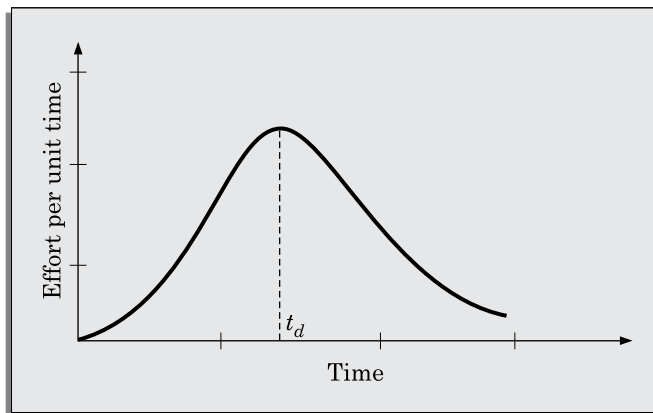
FIGURE 3.7 Rayleigh curve.
